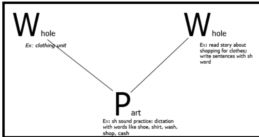
Figure 1: Whole-Part-Whole ( Trupke-Bastidas, 2007 )
